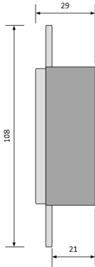
707WP2 Side
