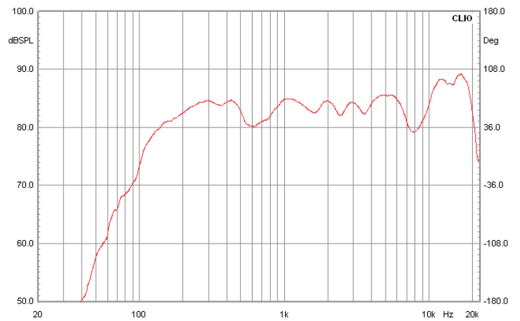
DA 180 Sens. 2.83V/1m: 85 dB (200-20k) half space
