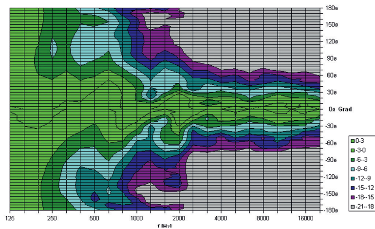
F 10 A vert. directivity plot
