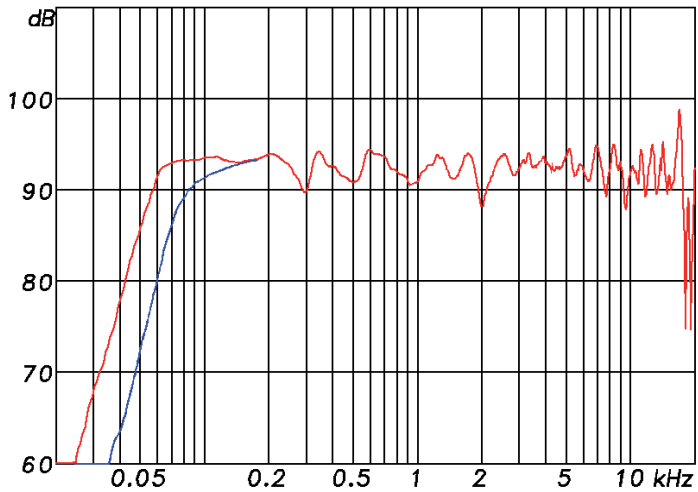
F 10 A hor. directivity plot
