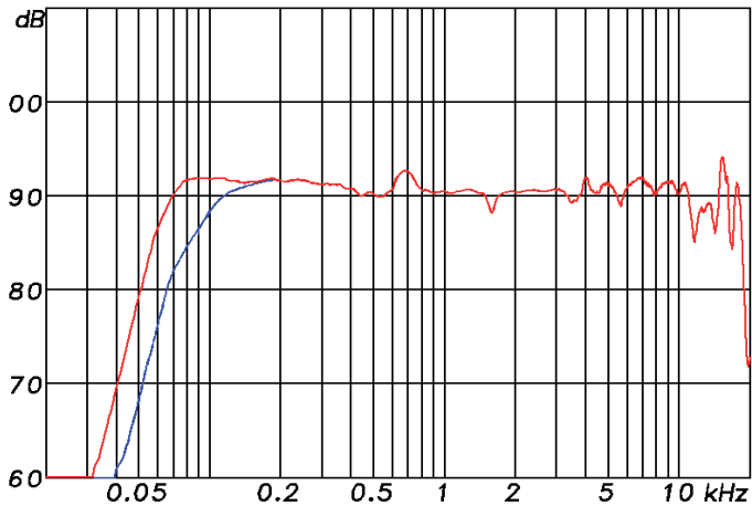
F 8 A hor. directivity plot
