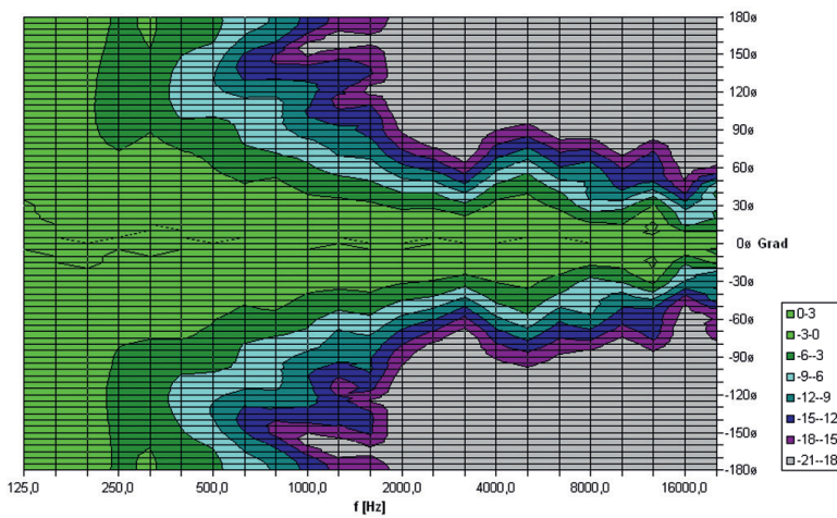
F 8 A vert. directivity plot
