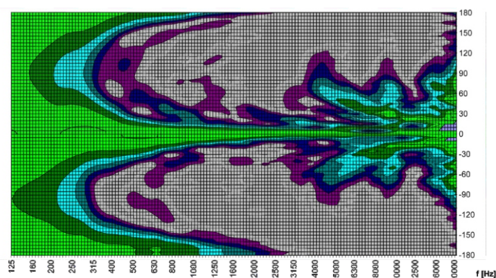
ZL 104 vert. Direktivity Plot
